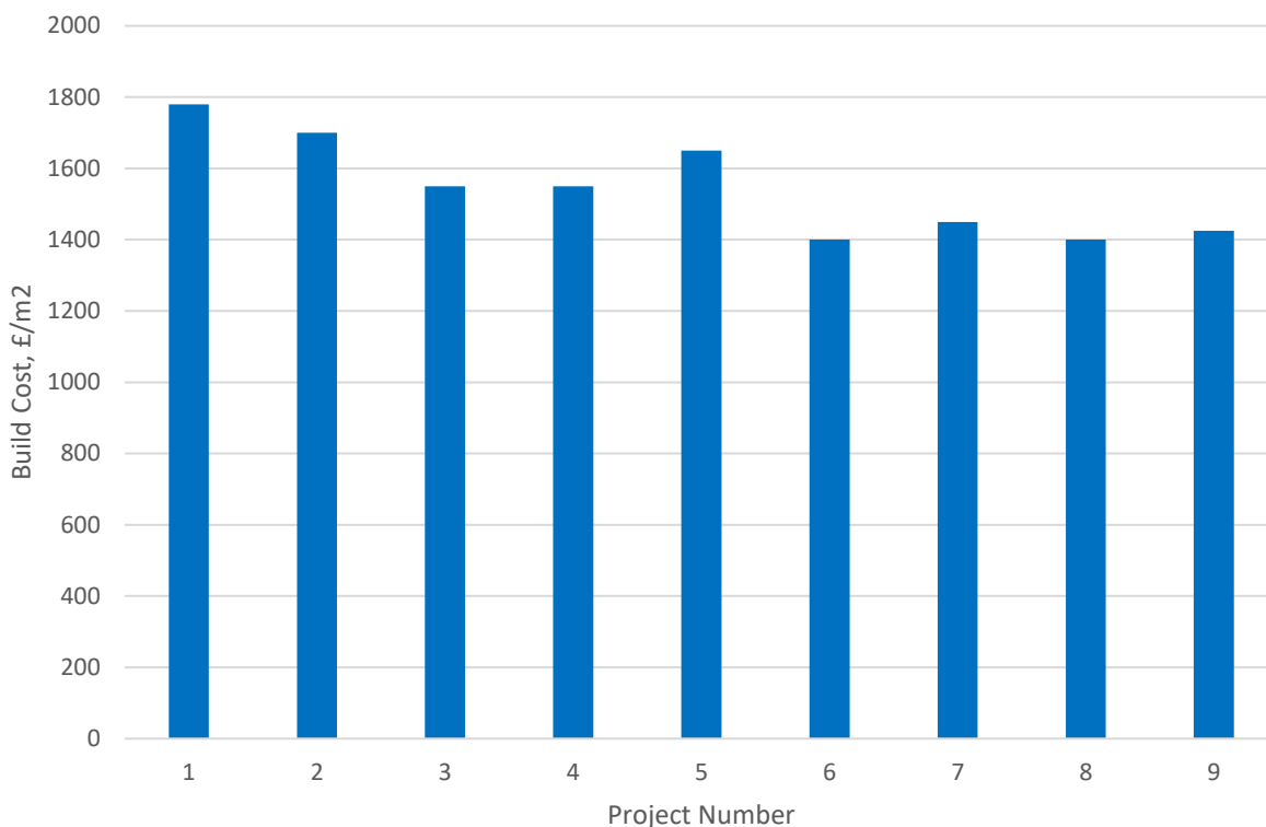
Costs of Exeter's Passivhaus housing developments over time, in £/m², adjusted for date, project size, and composition
